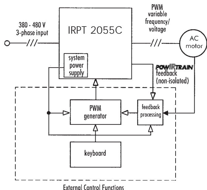
Figure 1. The IRPT2055C POWERTRAIN within a motor control system
